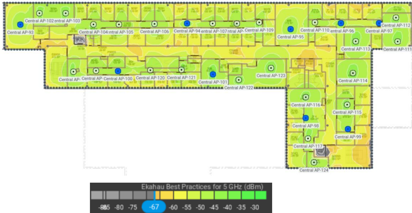
Central 3 rd floor 5GHz – After
