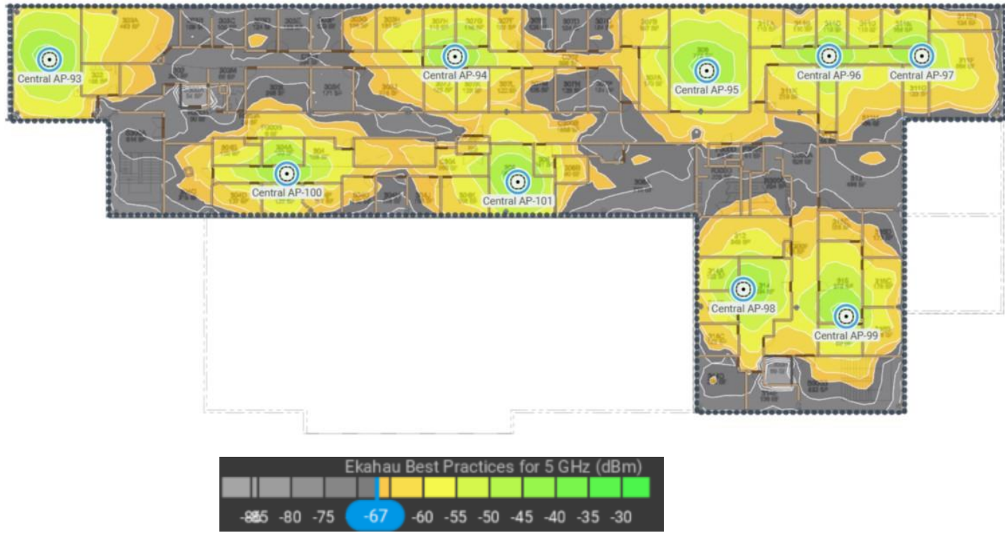
Central 3 rd floor 5GHz – Before
