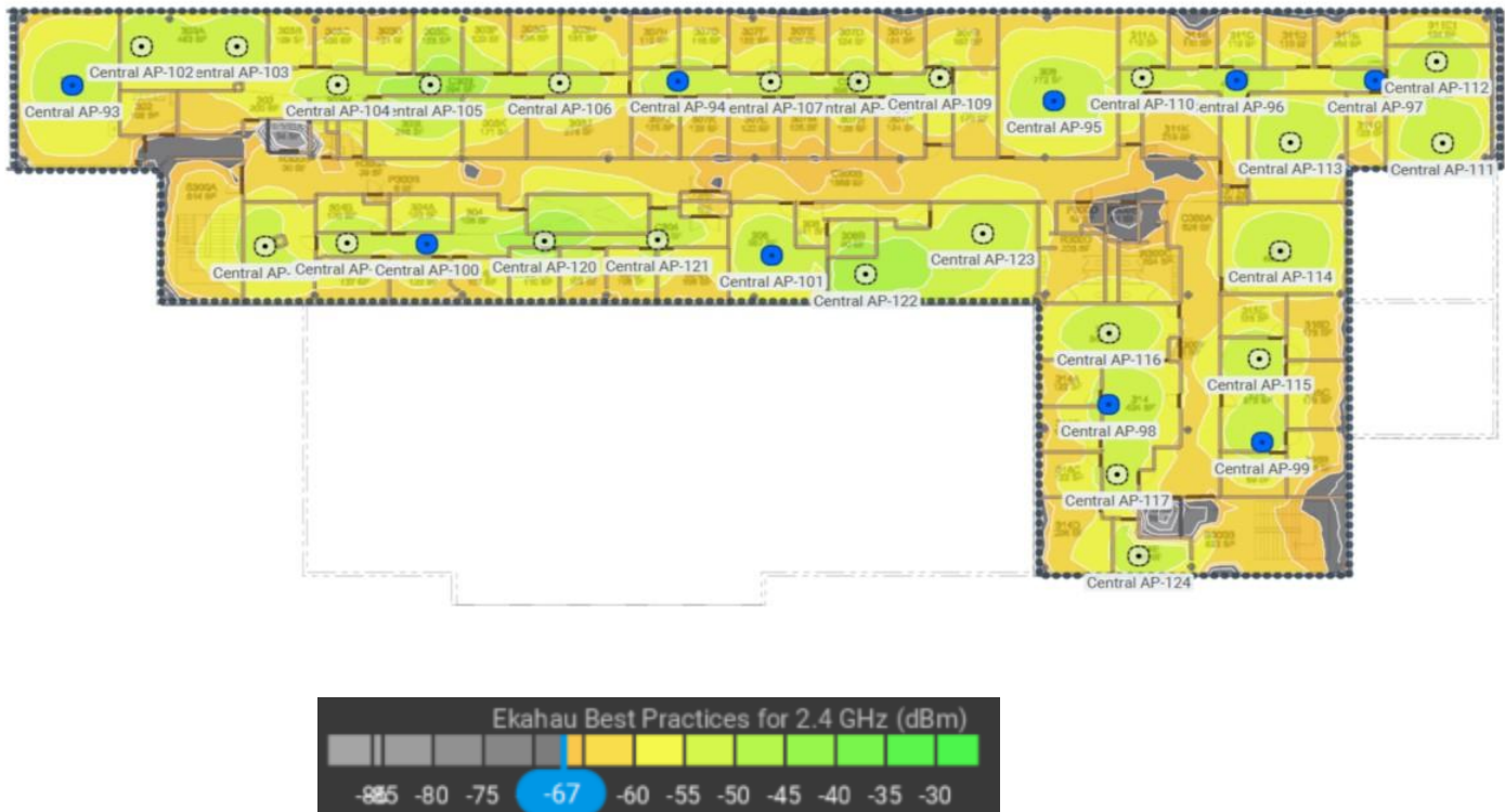
Central 3 rd floor 2.4GHz – After
