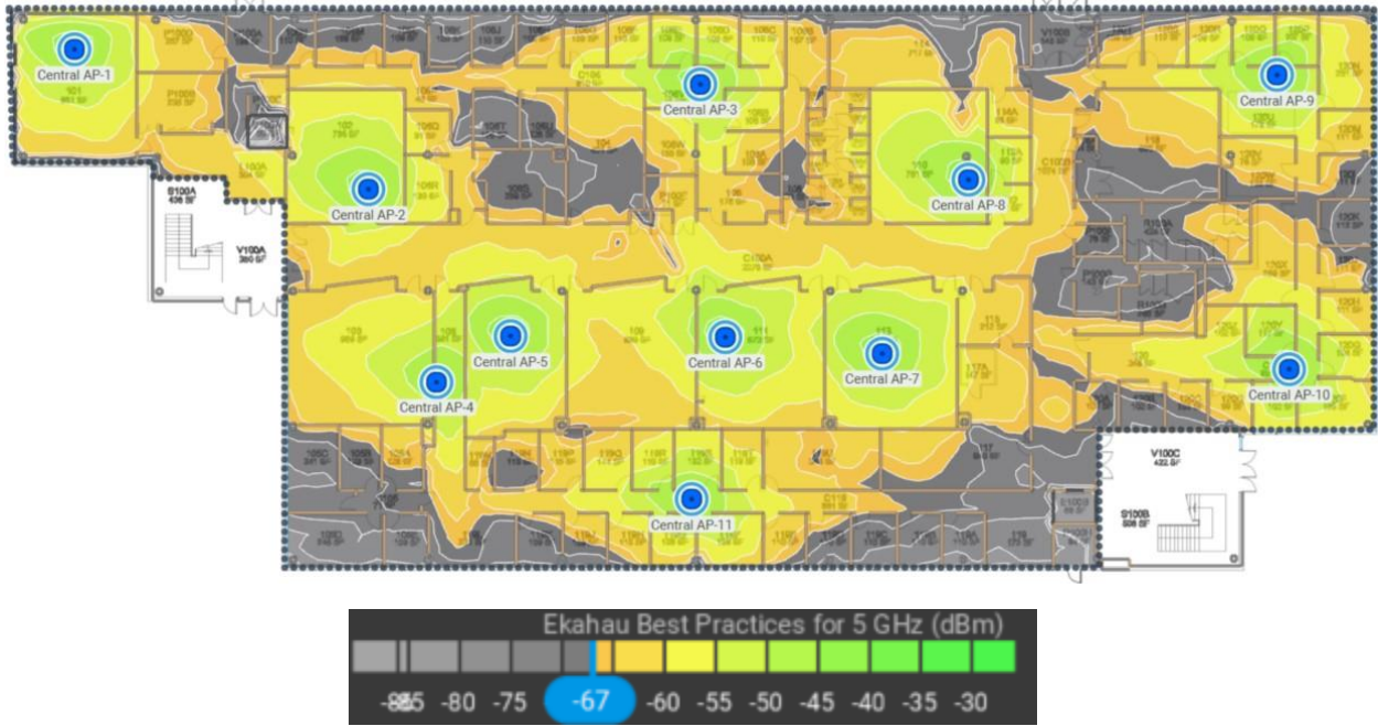
Central 1 st floor 5GHz - After
