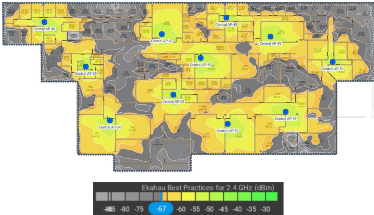
Central 2 nd floor 2.4GHz - After
