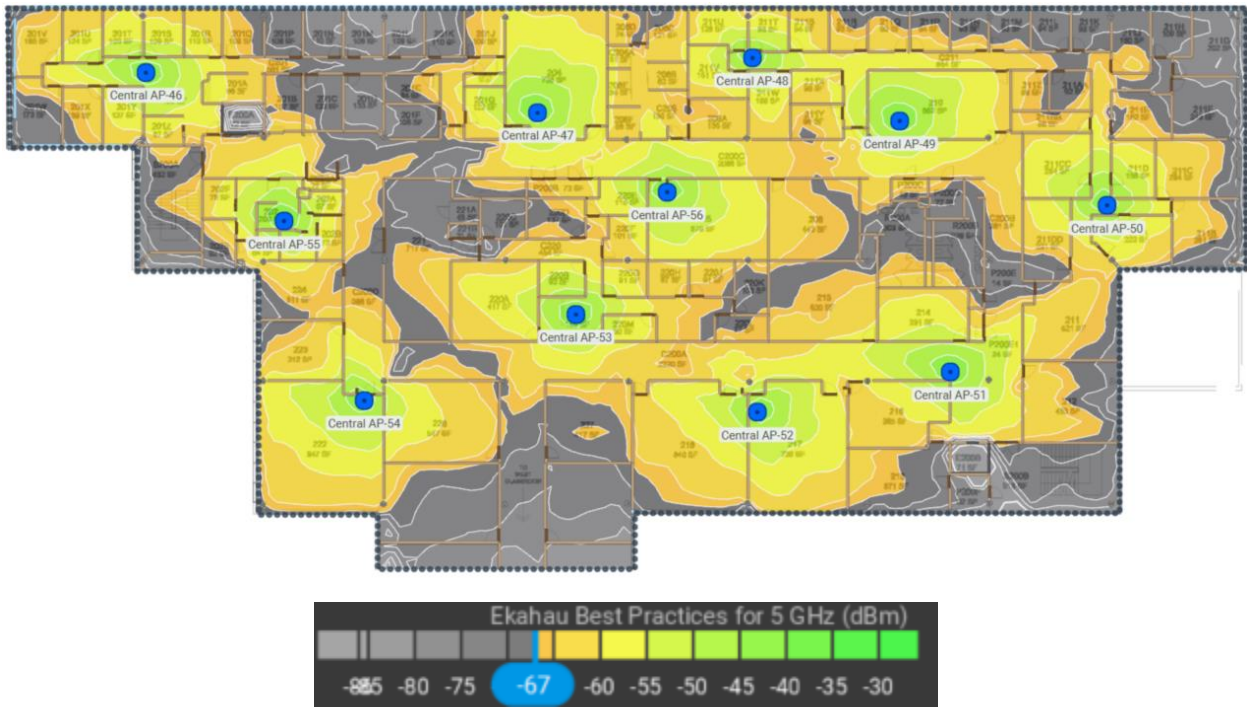
Central 2 nd floor 5GHz – Before
